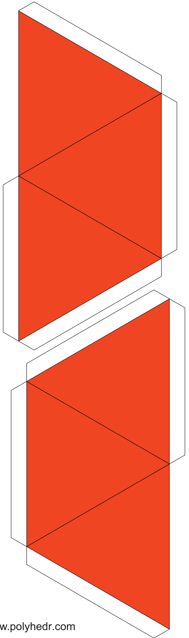
Stellated octahedron shape net
